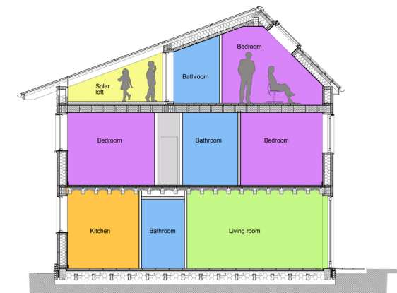
Cross Section
